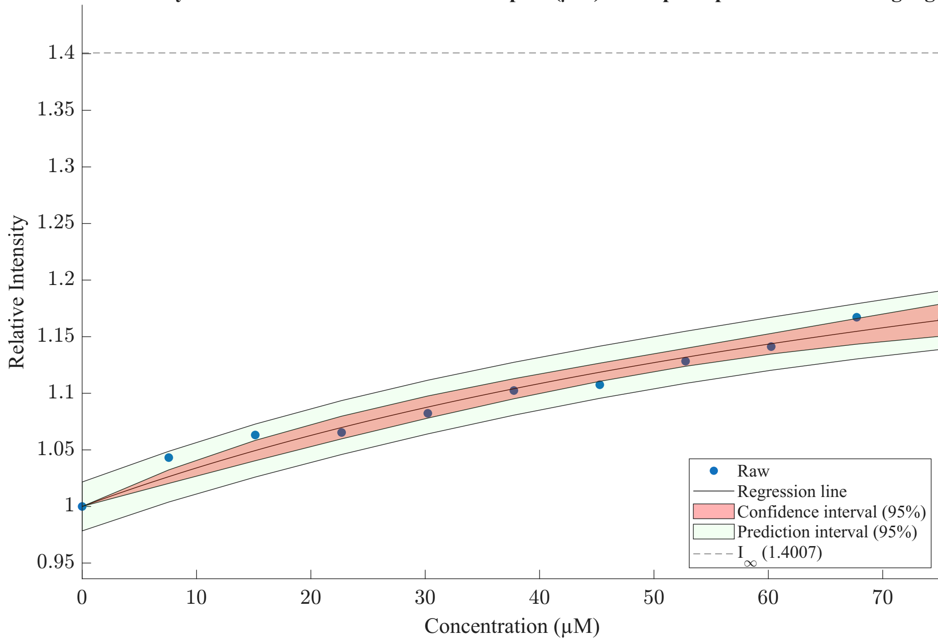
Relative intensity as a function of concentration of lipids ( \mu\text{M} ) for triple rep1 - Statistics fitting algorithm
